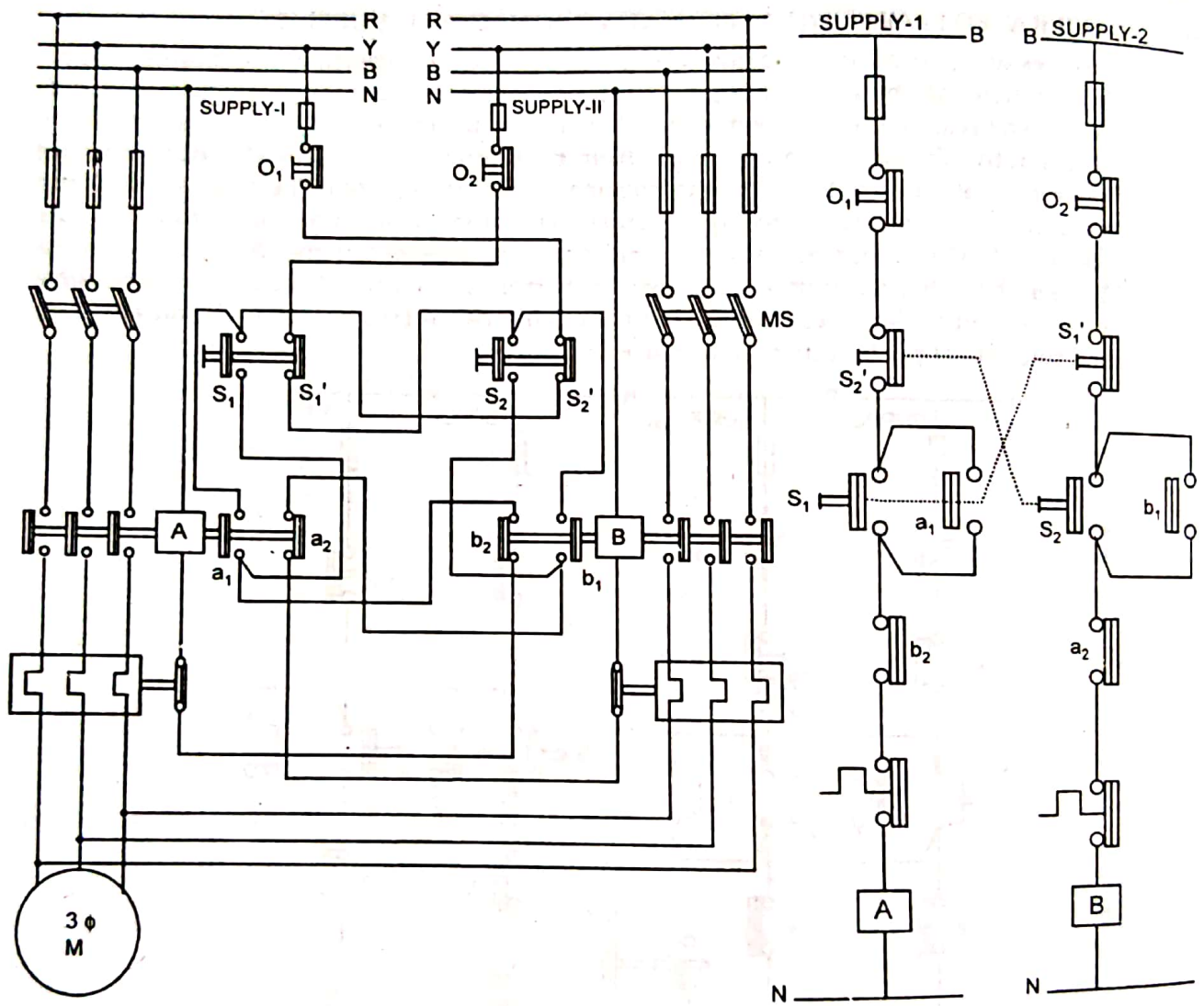
Fig. 7.31. Motor operated from two alternate sources of supply with additional mechanical locking.
