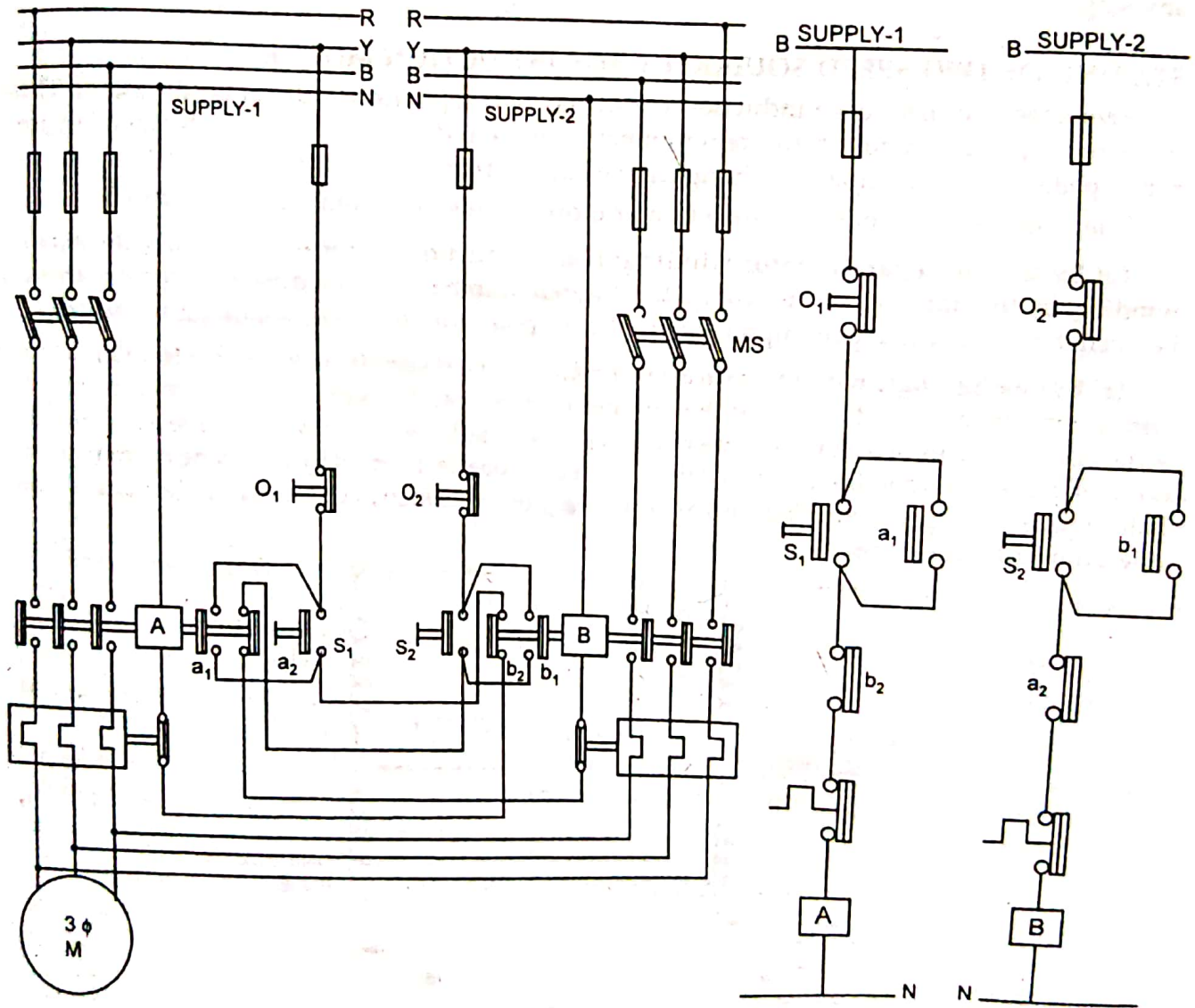
Fig. 7.32. Motor operated from two alternative source of supplies
